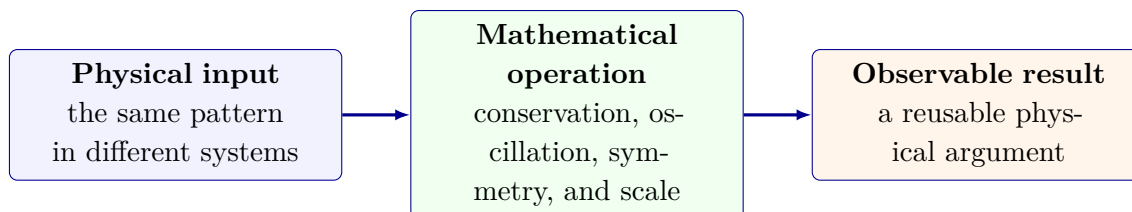
Figure 33.1: Visual model for connections across physics: the physical question becomes mathematics and returns as an observable prediction.
